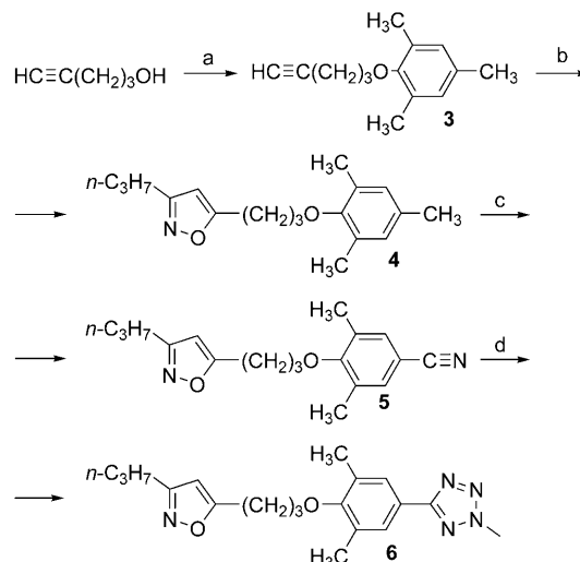
Scheme 1. Synthesis of a tetrazole analogue related to Disoxaril.
